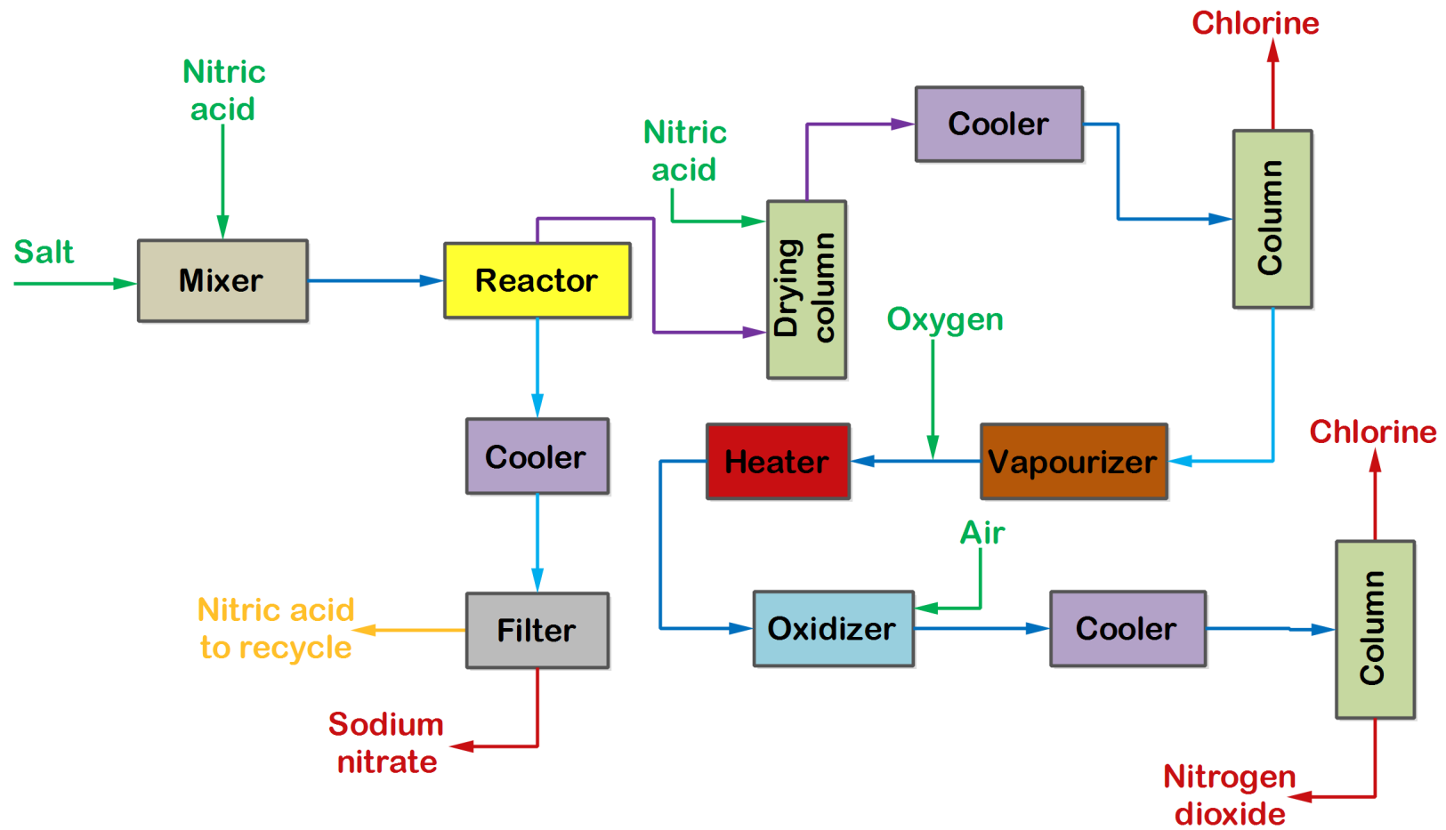
Figure: Manufacture of chlorine from salt and nitric acid
